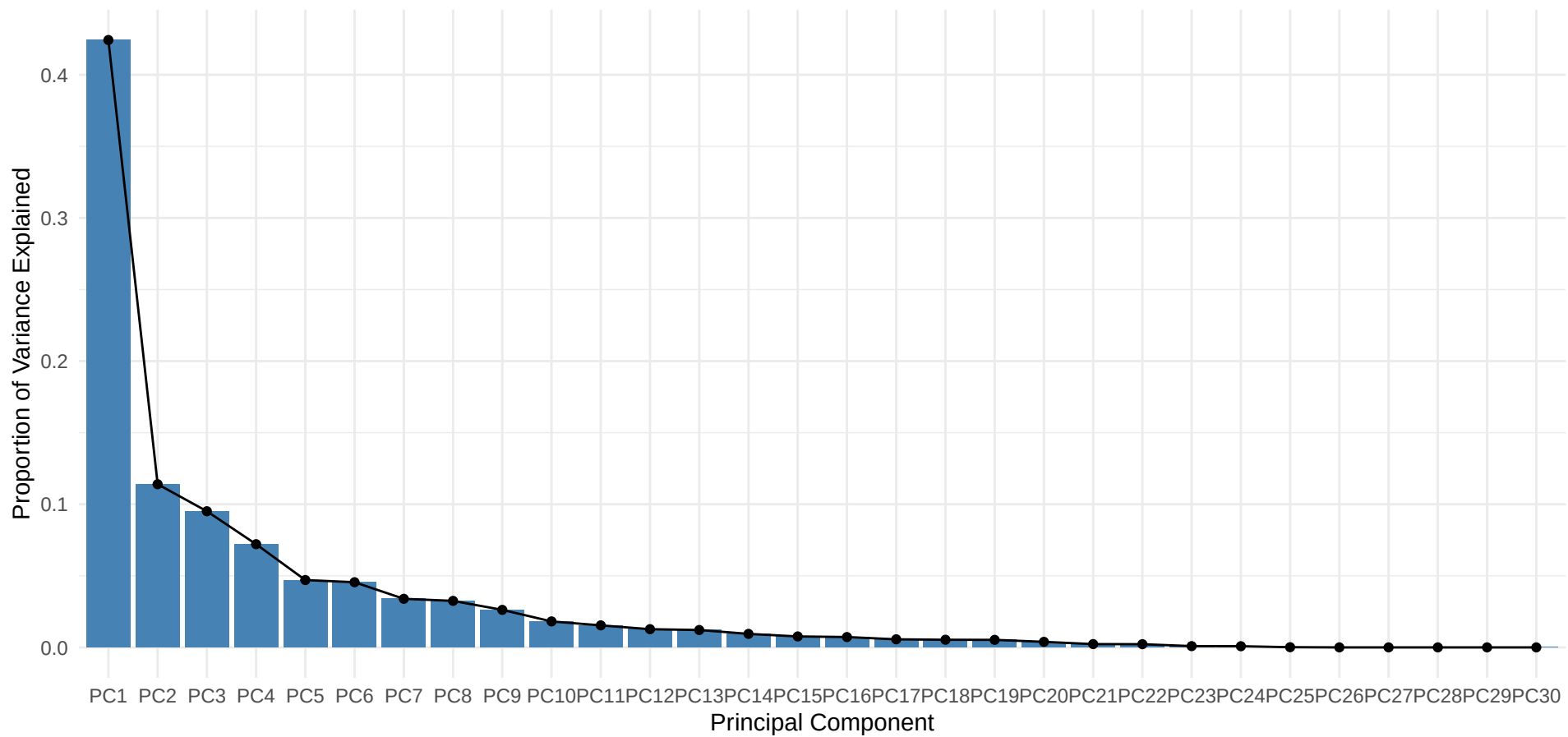
Scree Plot of PCA for FLARE002
